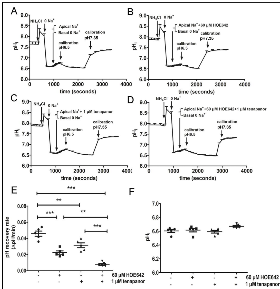
Fig. 6. Acid-activated apical Na + /H + exchange rates in differentiated C2PLKO.1 cells. In these experiments, the apical side of the cell monolayer was perfused with Na + -containing buffer A, while the basal side with Na + -free buffer C during the pH i -recovery period. (A) pH i curve of apical pH i recovery in the absence of inhibitors, (B) in the presence of 60 μM HOE642, (C) in the presence of 1 μM tenapanor, (D) in the presence of 60 μM HOE642 and 1 μM tenapanor in the apical perfusate in C2PLKO.1 cells. (E) Comparisons of acid-activated apical Na + /H + exchange rates without inhibitors, with 60 μM HOE642, 1 μM tenapanor, and 60 μM HOE642 plus 1 μM tenapanor. The total apical Na + /H + exchange rate of C2PLKO.1 cells was 0.046 ± 0.003 (ΔpH/min). 60 μM HOE642 reduced acid-activated apical Na + /H + exchange rates to 0.022 ± 0.002 (ΔpH/min), 1 μM tenapanor to 0.032 ± 0.003 (ΔpH/min), and 60 μM HOE642 plus 1 μM tenapanor to 0.008 ± 0.001 (ΔpH/min). (F) Comparisons of initial pH i at the beginning of acid-induced pH i recovery among different groups. (n=5, mean ± SEM, one-way ANOVA with Tukey's multiple comparison tests, **p< 0.01, ***p<0.0001).
