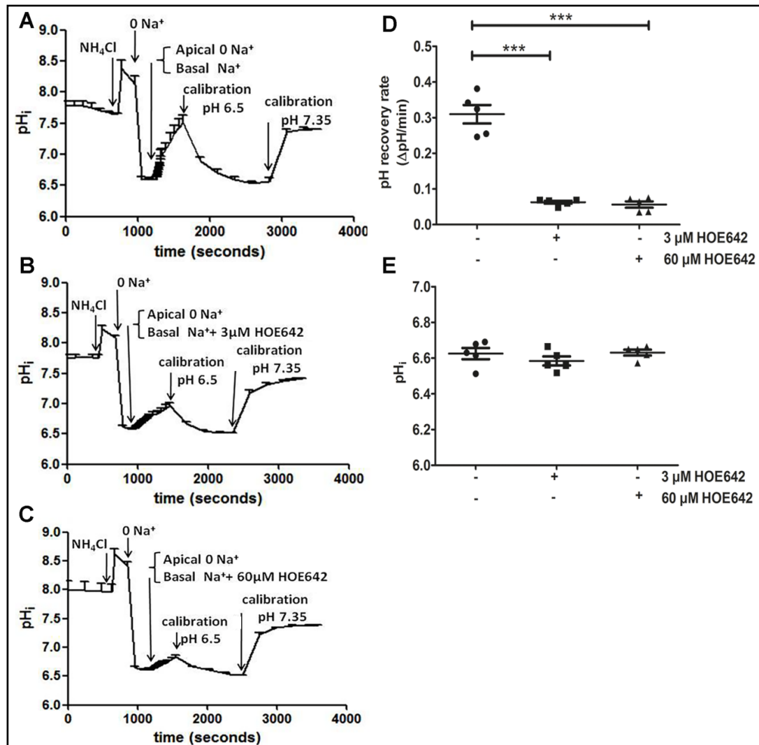
Fig. 5. Acid-activated basolateral Na + /H + exchange rates in differentiated C2PLKO.1 cells. C2PLKO.1 cells were acidified with the NH 3 /NH 4 + pre-pulse technique. During the recovery phase, the basal side of the cell monolayer was perfused with Na + -containing buffer A, while the apical side with Na + -free buffer C. Inhibitors were added 5 minutes before pH i recovery. (A) pH i curve of basolateral pH i recovery without inhibitors, (B) in the presence of 3 μM HOE642, (C) in the presence of 60 μM HOE642 in the basal perfusate in C2PLKO.1 cells. (D) comparisons of acid-activated basolateral Na + /H + exchange rates without inhibition and after 3 μM HOE642 and 60 μM HOE642 treatments. The total basolateral Na + /H + exchange rate of C2PLKO.1 cells was 0.310 ± 0.026 (ΔpH/min). 3 μM HOE642 reduced acid-activated basolateral Na + /H + exchange rates to 0.063 ± 0.004 (ΔpH/min), and 60 μM HOE 642 to 0.056 ± 0.009 (ΔpH/min). (E) Comparisons of initial pH i at the beginning of acid-induced pH i recovery among different groups. (n=5, mean ± SEM, one-way ANOVA with Tukey's multiple comparison tests, ***p < 0.0001).
