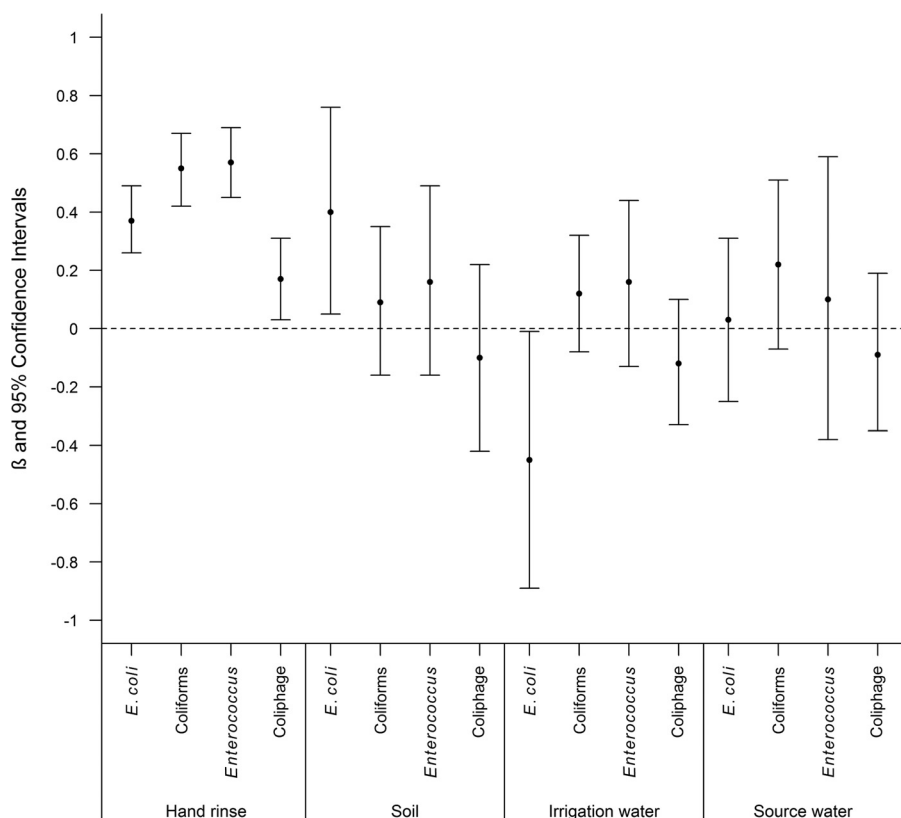
FIG 2 Linear model estimates ( \beta , represented by dots) and 95% confidence intervals (error bars) represent the \log_{10} change of the produce indicator concentration given a 1- \log_{10} increase in the matched environmental indicator concentration (hand rinse, soil, irrigation water, and source water). Models were adjusted for crop type (cantaloupe, jalapeño, and tomato), step in the production process (before harvest, after harvest, distribution, and packing facility), and year of sample collection (2011 or 2012). The dashed line indicates a linear estimate of zero. When the 95% confidence intervals cross the dashed line, this indicates a lack of statistical significance (i.e., P > 0.05 ). When the \beta and 95% confidence intervals do not cross the dashed line, they indicate a significant and positive (both are higher than the dashed line) or negative (both are lower than the dashed line) relationship.
