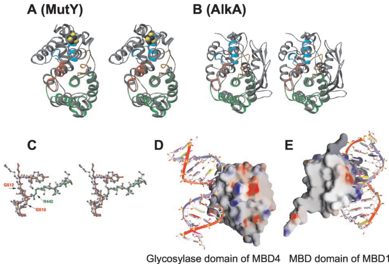
FIG. 3. Structural comparison of HhH glycosylases. A, superimposition of MBD4 glycosylase domain (colored according to Fig. 1B) and MutY (gray; Protein Data Bank code 1MUD). MutY (29), as well as EndoIII (30) and MIG (28), contains a C-terminal [4Fe-4S] cluster (shown in space-filling model). B, superimposition of MBD4 glycosylase domain and AlkA (gray; Protein Data Bank code 1DIZ). AlkA (26) and hOGG1 (27) contain an additional N-terminal \beta -sheet domain, and a 13- or 15-residue insertion between \alpha C and \alpha D (see Fig. 1B). C, superimposition of two DNA binding loops between MBD4 (red and green) and AlkA (gray). The Gly-rich hairpin loop of HhH motif is indicated by conserved Gly 510 and Gly 512 of MBD4. The minor groove wedge (Leu 125 in AlkA), which assists in base flipping, superimposed on Arg 442 of MBD4 in the loop between helices \alpha B and \alpha C (see Fig. 1B). D, based on the superimposition shown in C, the MBD4 glycosylase domain is docked to DNA from the minor groove side. E, the MBD domain of MBD4 has not yet been structurally characterized; however, the NMR solution structure of the MBD domain of MBD1 was shown to bind DNA from the major groove side (13).
