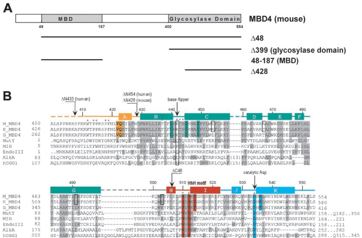
FIG. 1. A , schematic representation of mouse MBD4. Two stable fragments ( shaded ) were identified by limited proteolysis. Below the full-length mouse MBD4 are the depicted protein fragments ( \Delta 48 , MBD, glycosylase domain \Delta 399 , and \Delta 428 ) used in this study. B , structure-guided sequence alignment of three MBD4 glycosylase domains (mouse, AAC68878; human, AAC68879; and Gallus, AAF68981) and five HhH glycosylases. We note that the reported MBD4 homolog in chickens only contains the glycosylase domain and has no consensus sequence for the N-terminal MBD (10). The secondary structure of MBD4 is indicated above the sequence and colored the same as in Fig. 2A. The dashed lines indicate the gaps introduced to optimize alignments, and MBD4 has the shortest loop prior to the HhH motif. The dots indicate extra residues outside the glycosylase domain. The residues in the active site, proposed to interact with the extrahelical target nucleotide, are colored to match their associated region. The residues marked by * above the sequence are discussed in the text. The deletion mutants made in human MBD4 (10, 33) and mouse MBD4 (this study) are indicated by arrows . The four differences between mouse and human MBD4 sequences are boxed .
