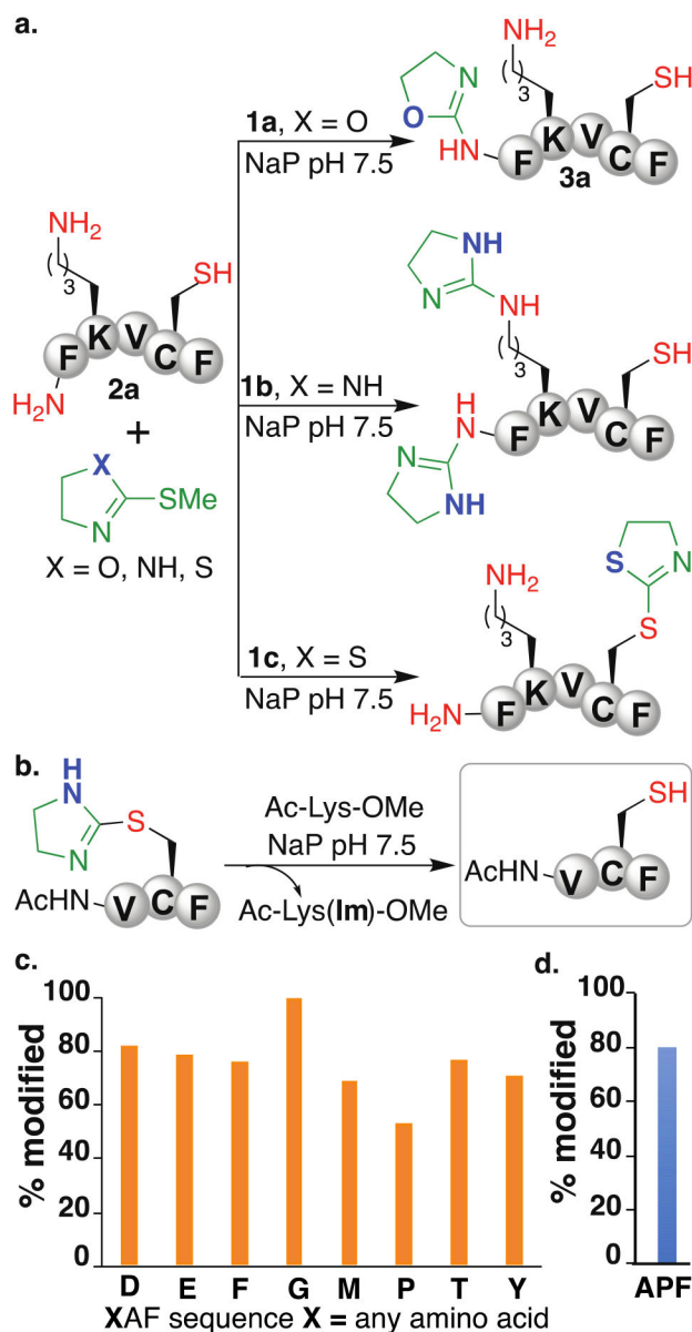
Figure 2. Site-selective polypeptide modification using azolines. a. Screening of various azolines such as oxazoline 1a , imidazoline 1b and thiazoline 1c to determine their chemoselectivity for peptides. b. Reversibility of azoline-cysteine adduct with lysine. c. Universal sequence compatibility of peptides with azolation. Conditions for a–b : 4 mM peptide, 200 mM azoline, 10 mM phosphate buffer at pH 7.5 and 37 °C. Conditions for c : 6.25 mM peptide, 312.5 mM 1a , Ox1 , 10 mM phosphate buffer at pH 7.5 and 37 °C for 3 h.
