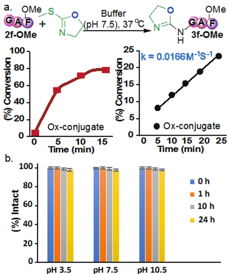
Figure 3. Rate and stability studies of oxazolation. a. Rate studies for synthesis of Ox-GAF-OMe conjugate 3f-OMe . b. The oxazolation of tripeptide GAF-OMe 2f-OMe (1 mM) with 1a (1 mM) at pH 7.5 follows a second order rate constant. b. pH stability of Ox-GAF-OMe conjugate 3f-OMe at 25 °C.
