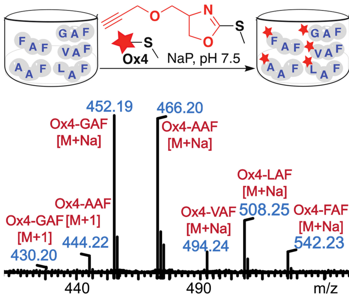
Figure 5. Selective N-terminal labelling of all the peptides by oxazoline Ox4 in the complex mixture of a variety of peptides.
